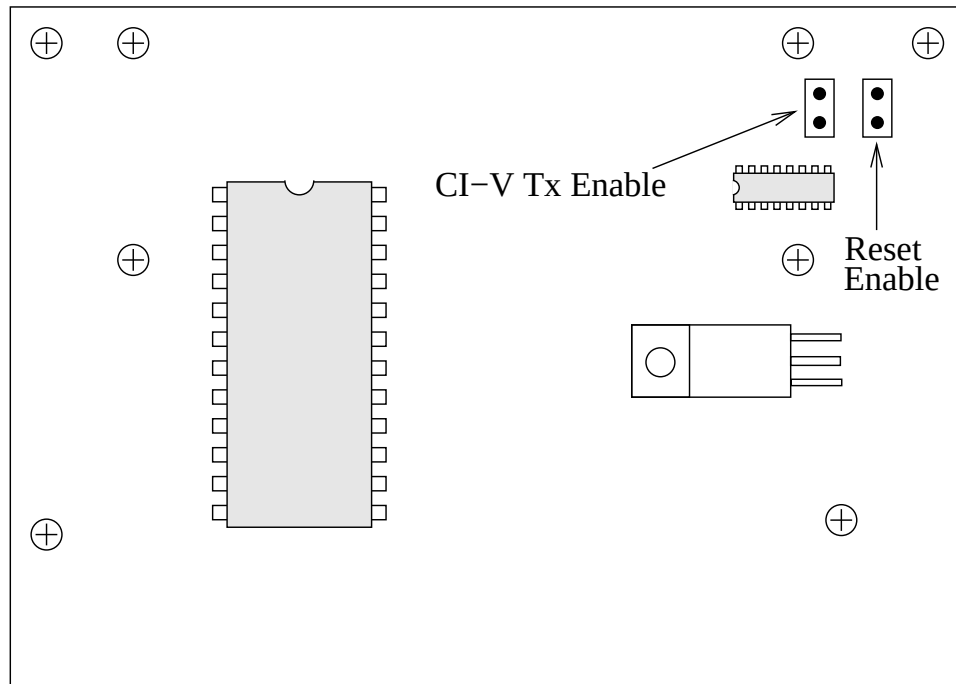
Figure 12.1: Jumper Locations
